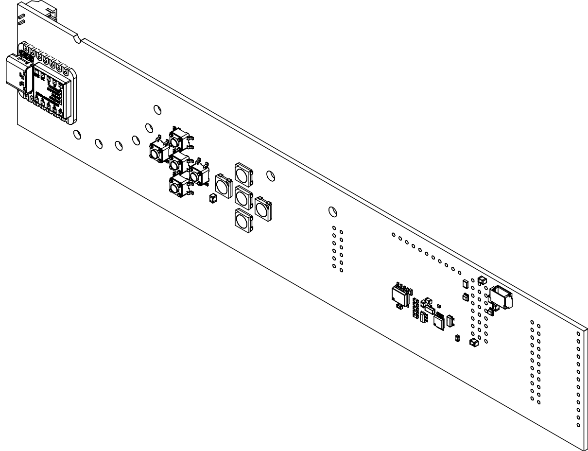
View from Top side (Scale 1:1)
