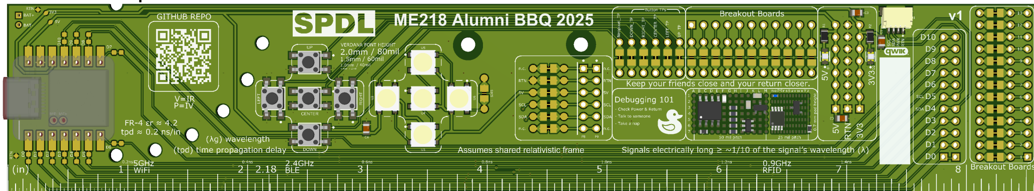
Realistic View: Top side
